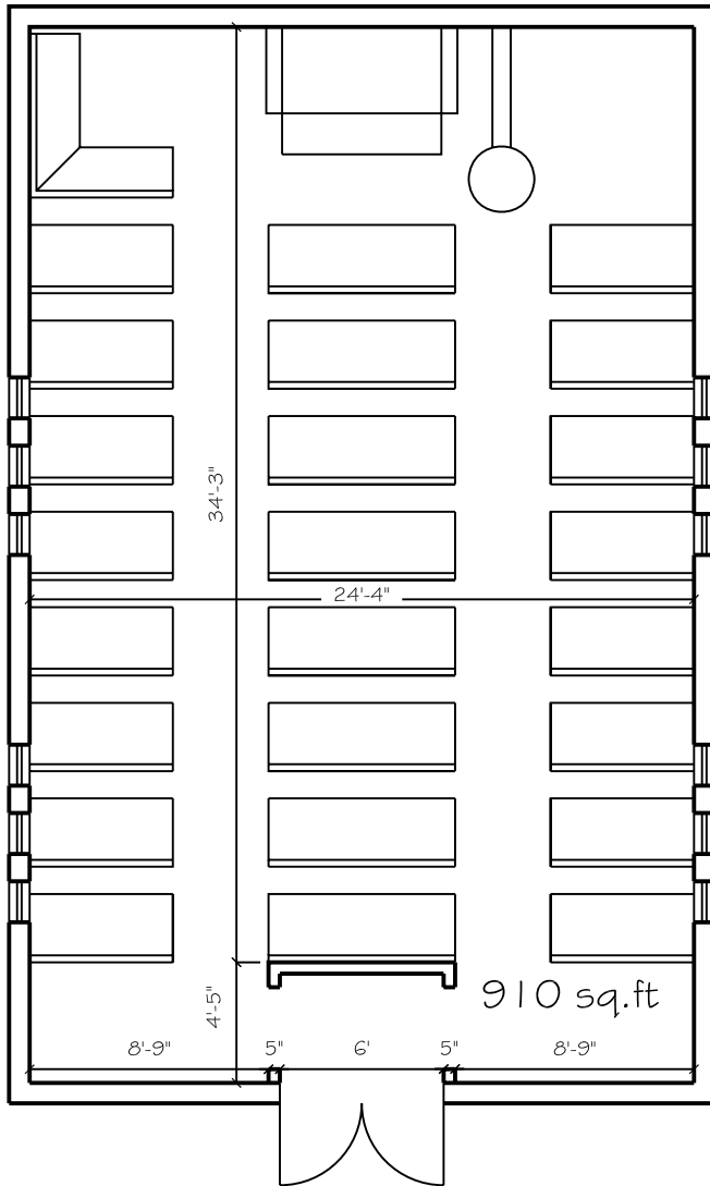
FLOOR PLAN
